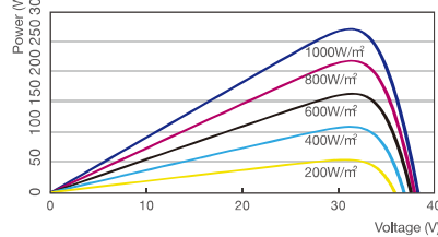
Power-Voltage Curve FXN285P-60
