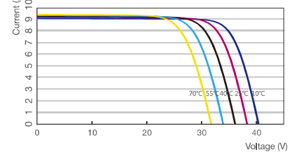
Current-Voltage Curve FXN285P-60
