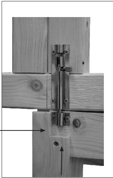
Ruuvi 4x25mm
