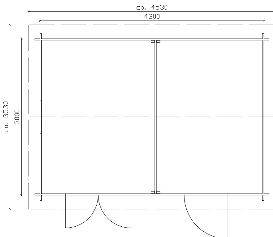
Lillevilla 12-2: 4100 x 3000 mm
