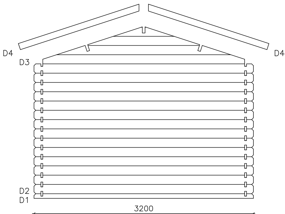
Lillevilla 12-2: 4100 x 3000 mm
