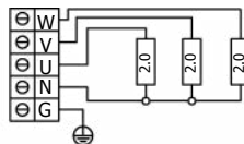
DRFT3-60NS-WL 6,0 kW
