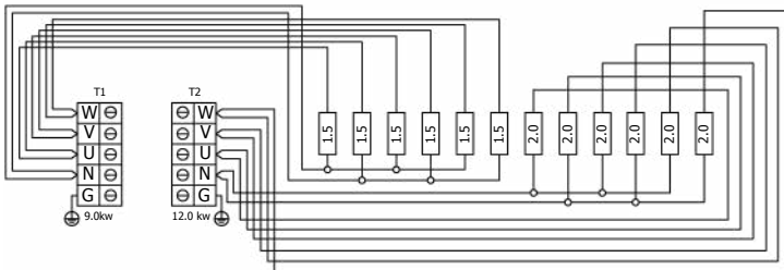
DRFT12-210NS-WL 21,0 kW
