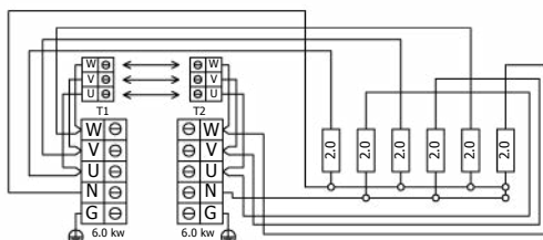
DRFT6-120NS-WL 12,0 kW
