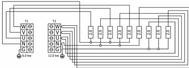
DRFT9-180NS-WL 18,0 kW
