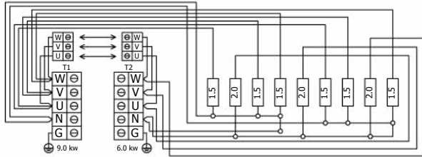
DRFT9-150NS-WL 15,0 kW
