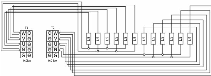
DRFT12-180NS-WL 18,0 kW
