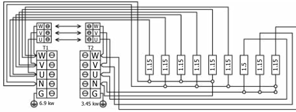
DRFT9-105NS-WL 10,5 kW
