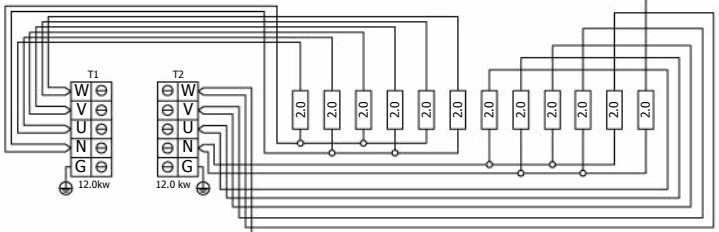
DRFT12-240NS-WL 24,0 kW
