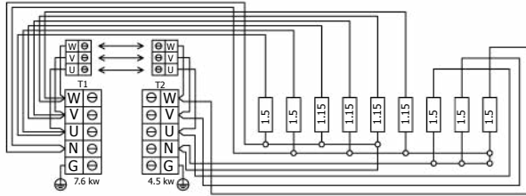
DRFT9-120NS-WL 12,0 kW
