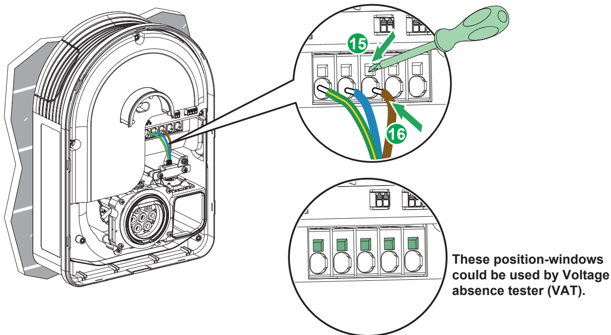
iMNx/TIC/DSO wiring
