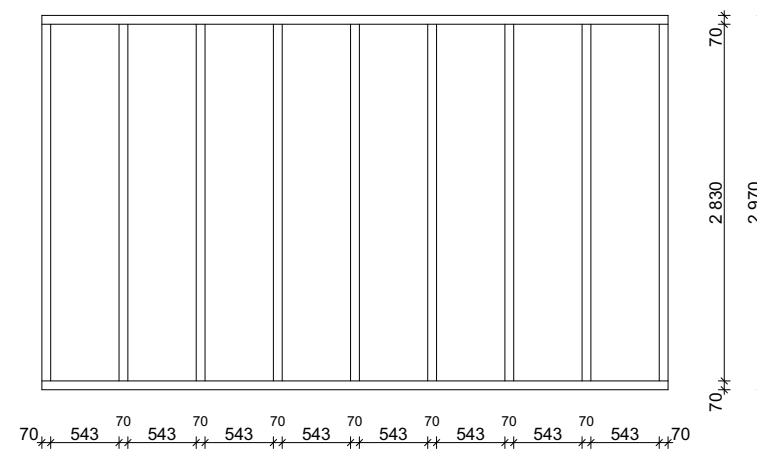
Foundation view
