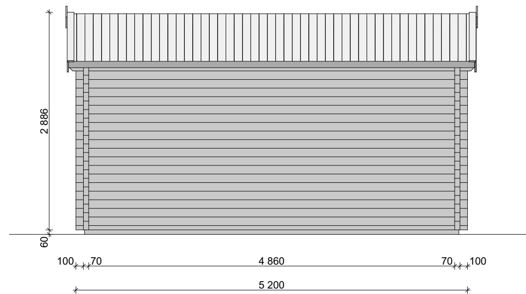
Rear view
